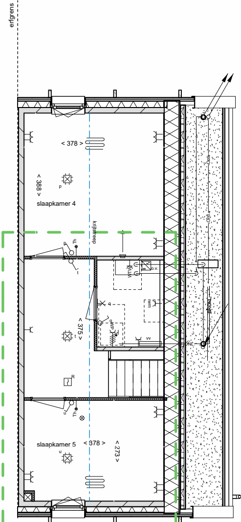
zolder
