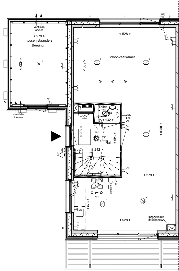
00 begane grond
